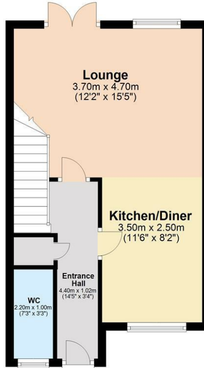
Ground Floor Approx. 36.2 sq. metres (389.9 sq. feet)
